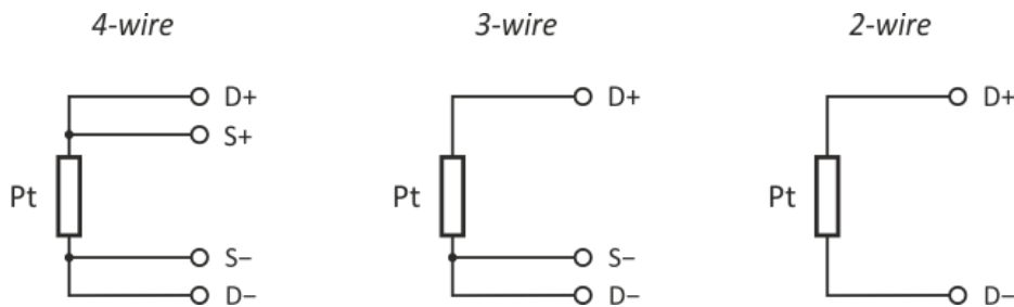
fig. 1 – Connecting Pt sensor based on the sensor wiring
