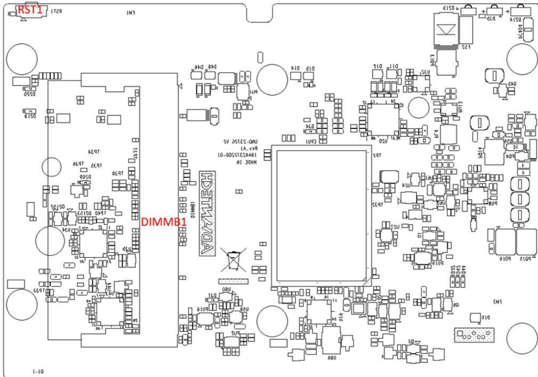
Figure 2.5 Diagram of Key Components Location on UNO-2372G V2 (Bottom Side)
