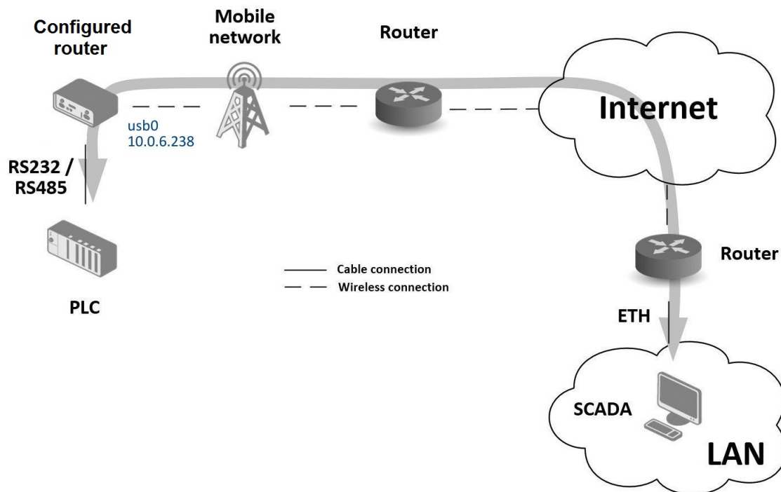
Figure 100: Serial Gateway – sample topology
