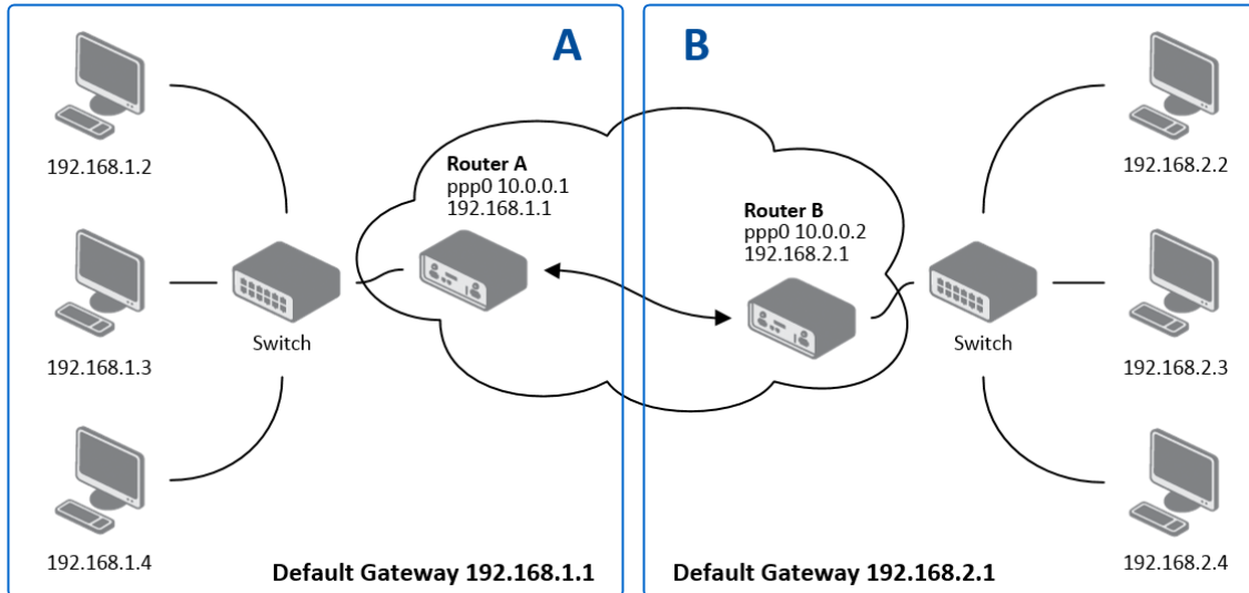
Figure 49: Topology of L2TP Tunnel Configuration Example
