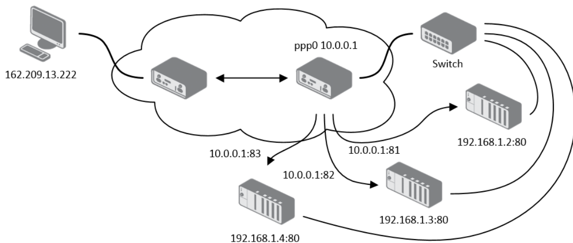
Figure 40: Topology for NAT Configuration Example 2
