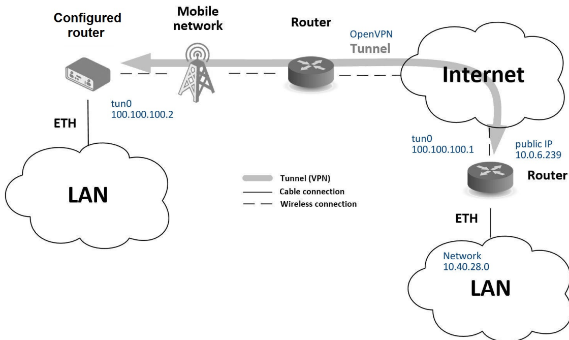
Figure 98: Secure networks interconnection – sample topology
