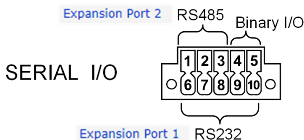
Figure 68: SERIAL I/O configuration pages overview
