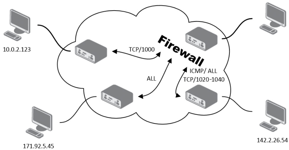
Figure 35: Topology for the IPv4 Firewall Configuration Example
