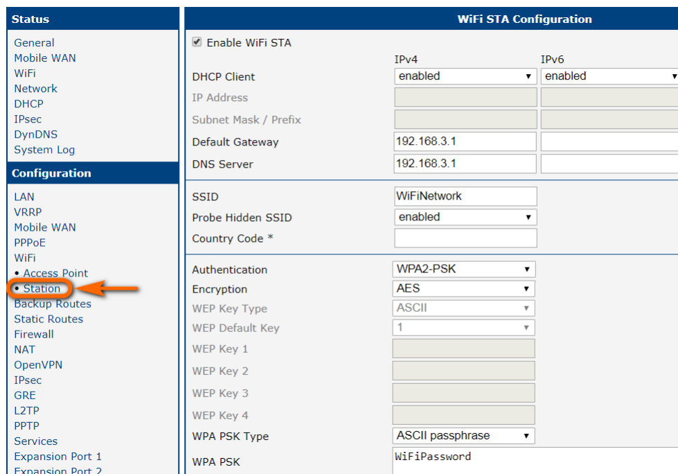
Figure 95: Backup access to the Internet – WiFi configuration
