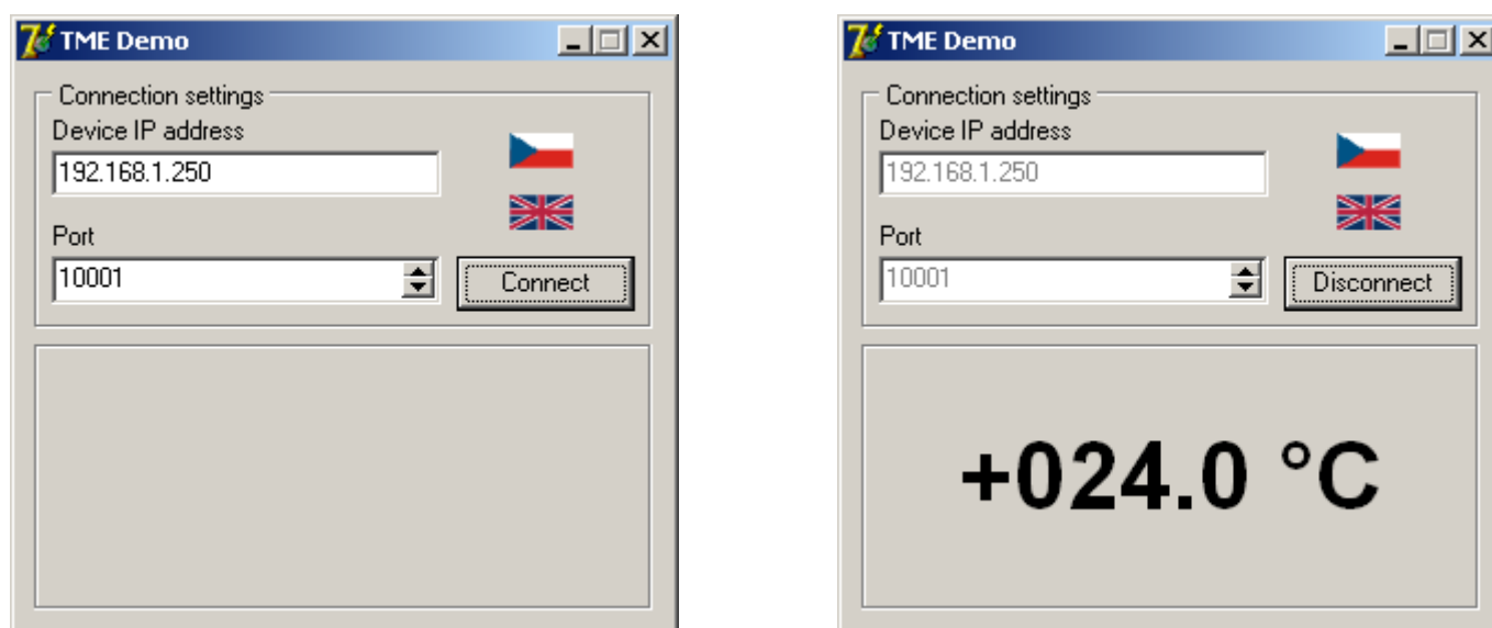
Fig. 29 – demo program
