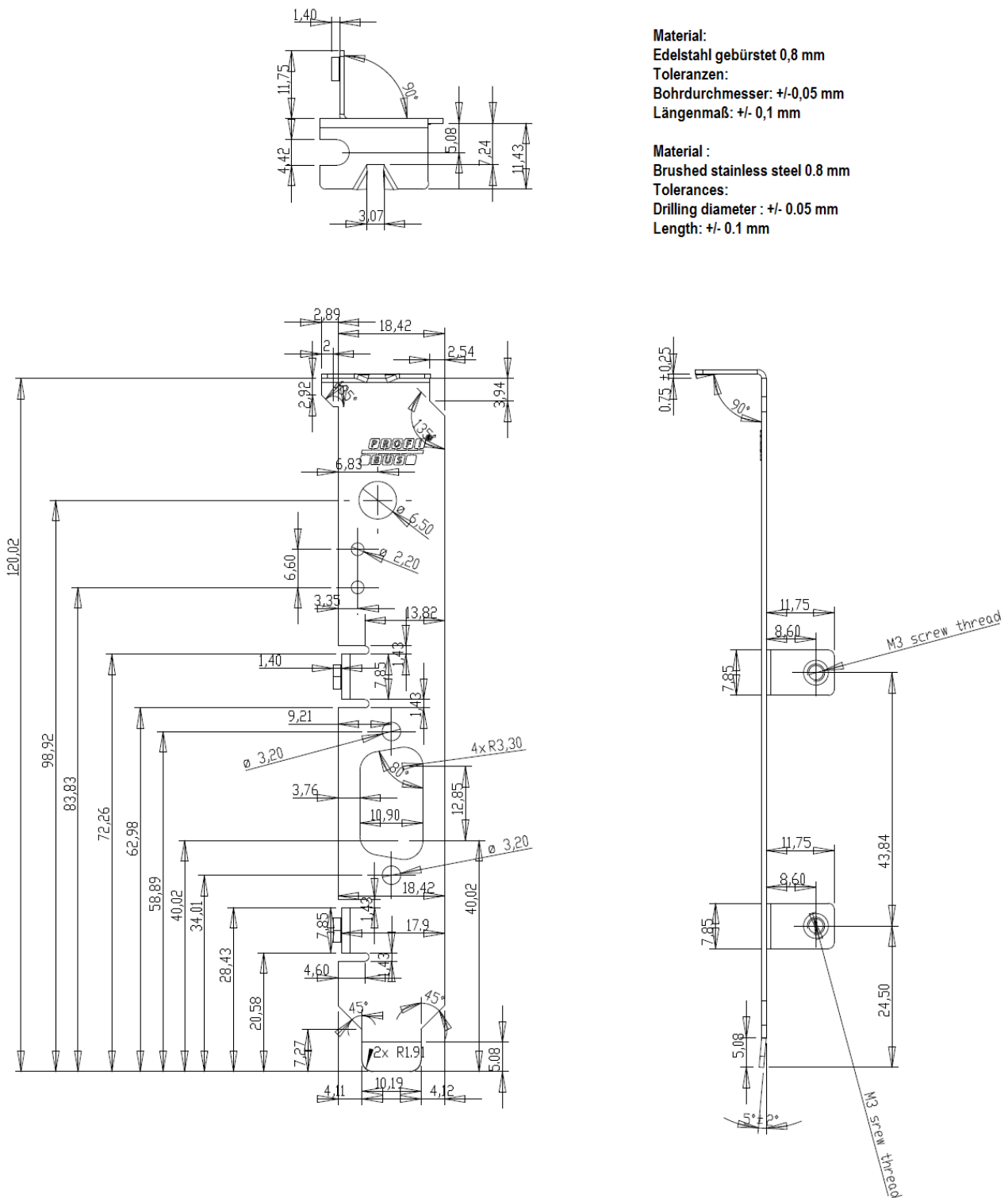
Figure 74: Dimensions Front Panel CIFX 50-DP or CIFX 50E-DP
