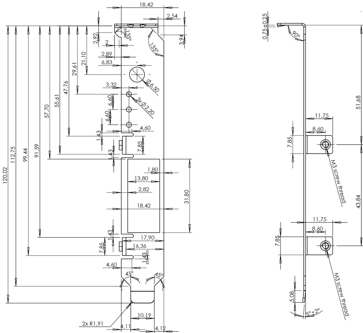
Figure 69: Dimensions Front Panel CIFX 50-RE, CIFX 50E-RE or CIFX 50E-REIET
