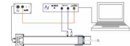
Impedance Tube System for Sound Absorption Measurement
