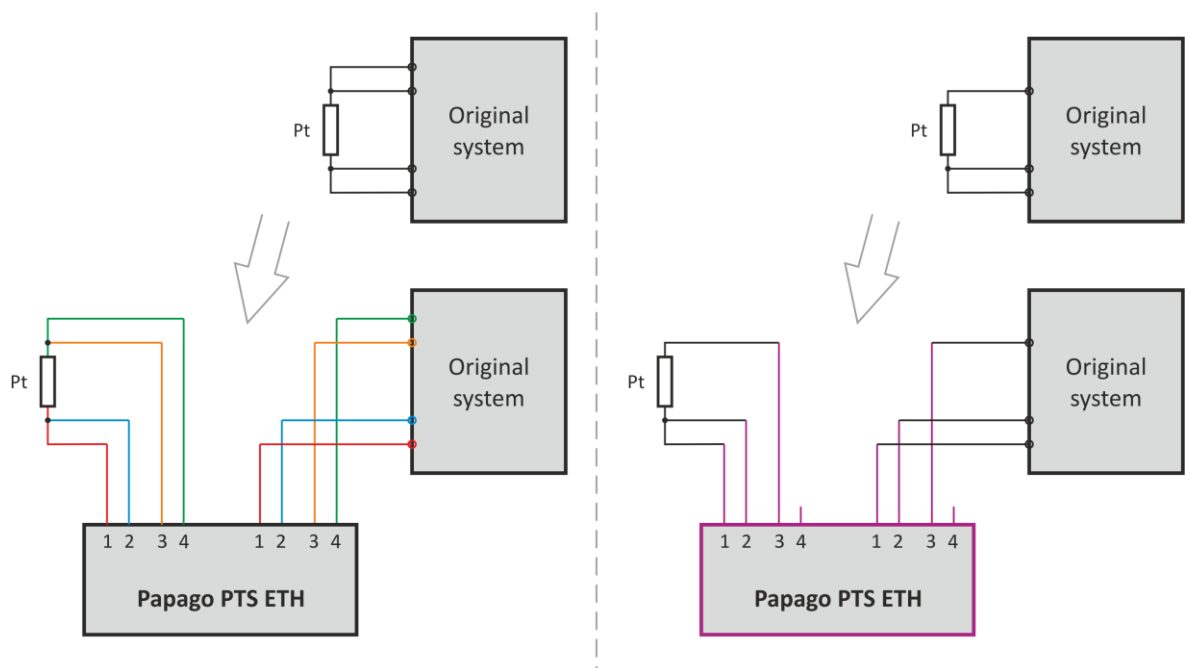
fig. 2 - Connecting Papago into the existing system (via four wires - right, or three wires - left)
